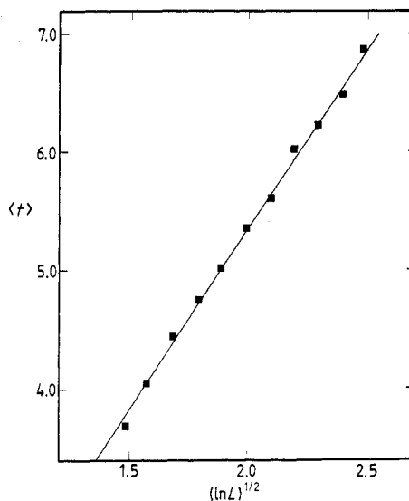
Figure 1. Variation of average time \langle t \rangle for a lattice to reach state 29 at all sites, if initially a random fraction p = 0.125 of sites are in state 1 (killer cells), and the others in state zero (healthy). Four thousand lattice configurations of size N = L^2 were simulated for each L . Note the logarithmic scale for N . No sites were taken as inert. The size of the squares represents the size of the error bars.
